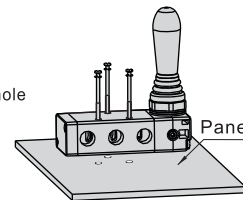
Body Installation
